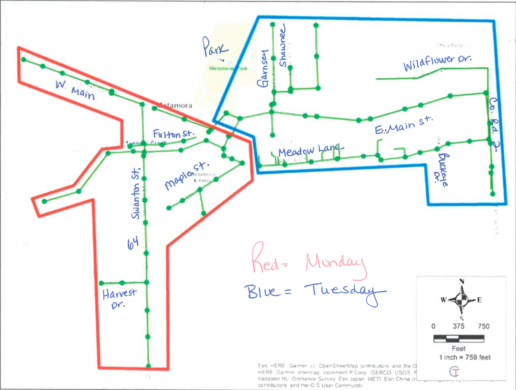
Village of Metamora - Sanitary Collection System
